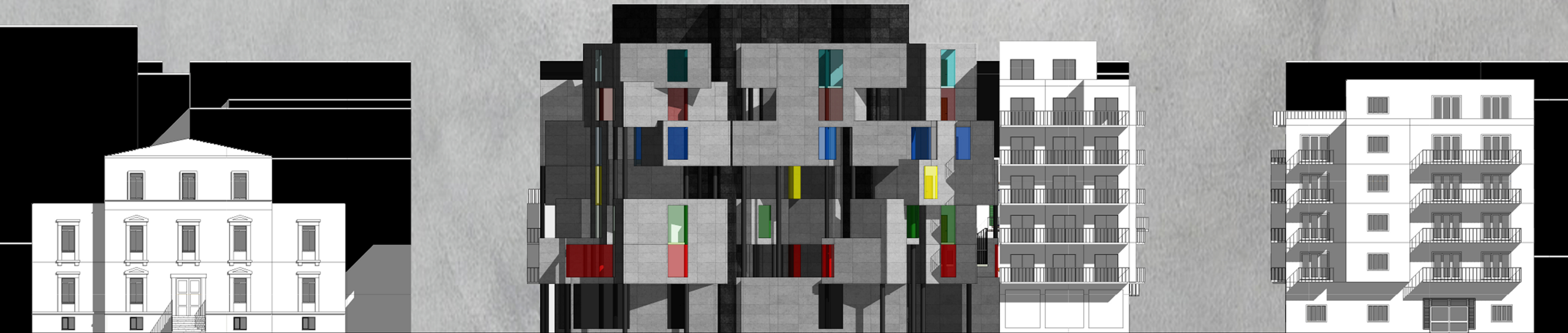
South Elevation 1:100
