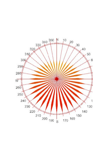
Diffuse Radiation(kWh/m2) Milano_Linate_ITA_2005 1 JAN 1:00 - 31 DEC 24:00
