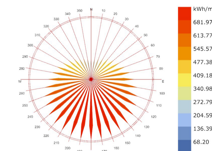
Total Radiation(kWh/m2) Milano_Linate_ITA_2005 1 JAN 1:00 - 31 DEC 24:00
