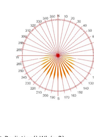
Direct Radiation(kWh/m2) Milano_Linate_ITA_2005 1 JAN 1:00 - 31 DEC 24:00
