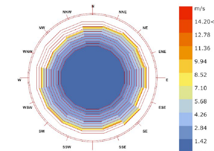
Wind-Rose Milano-Linate_ITA 1 JAN 1:00 - 31 DEC 24:00 Hourly Data: Wind Speed (m/s) Calm for 61.24% of the time = 5365 hours.
