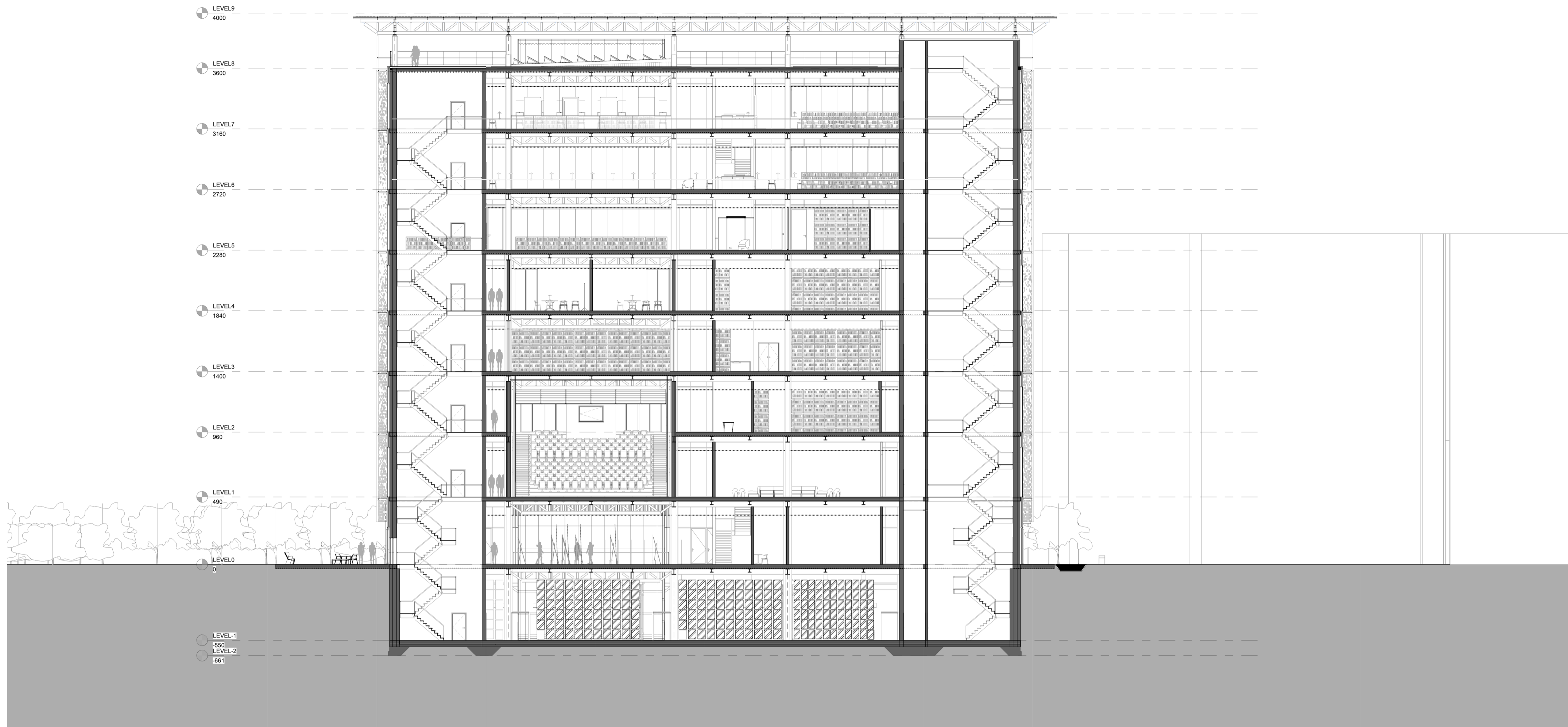
TRANSVERSE SECTION - through the auditorium
