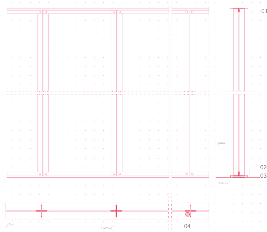
Type A. module (permeable version) basic module for swiveling doors
