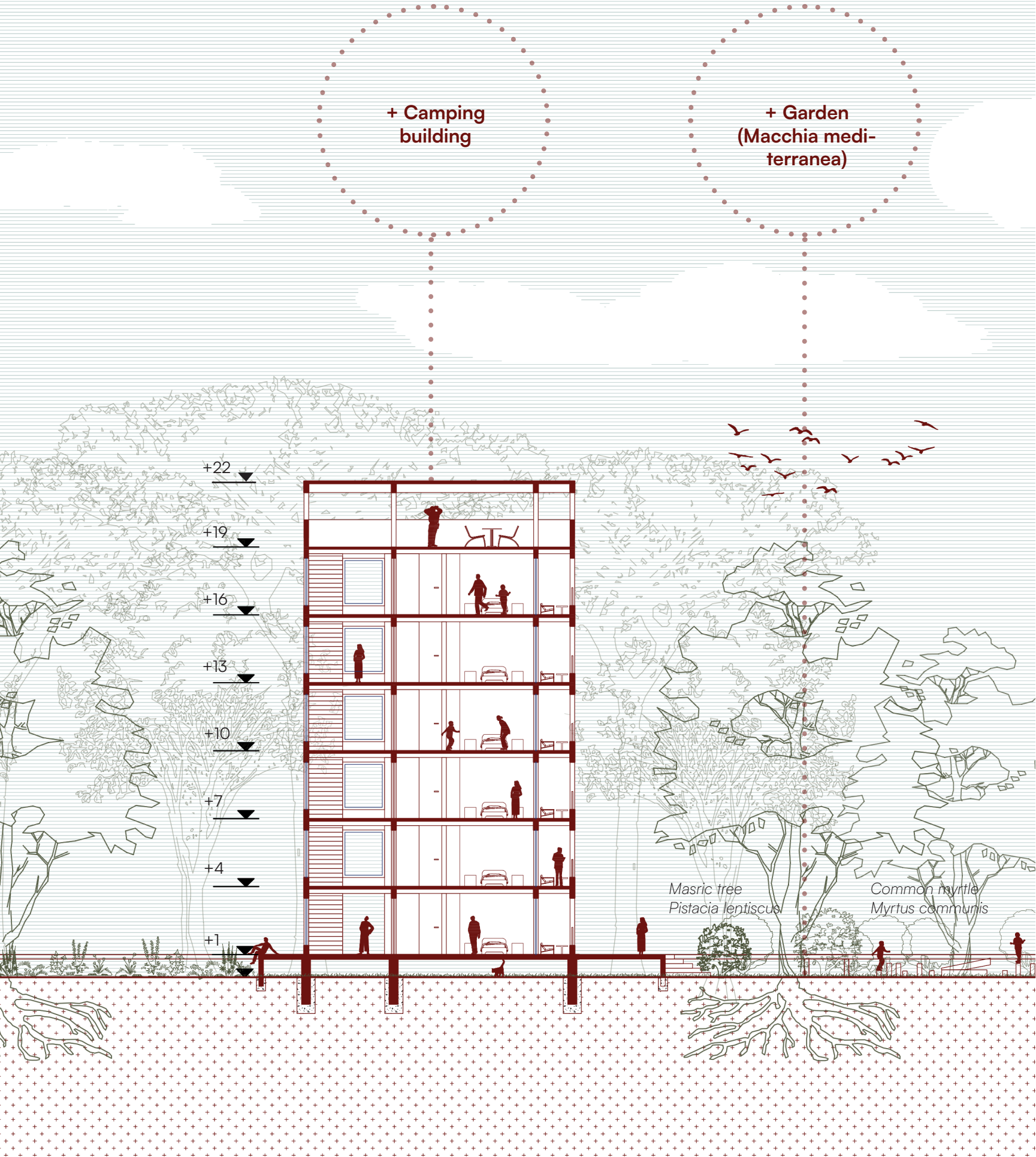
Section B-B'
